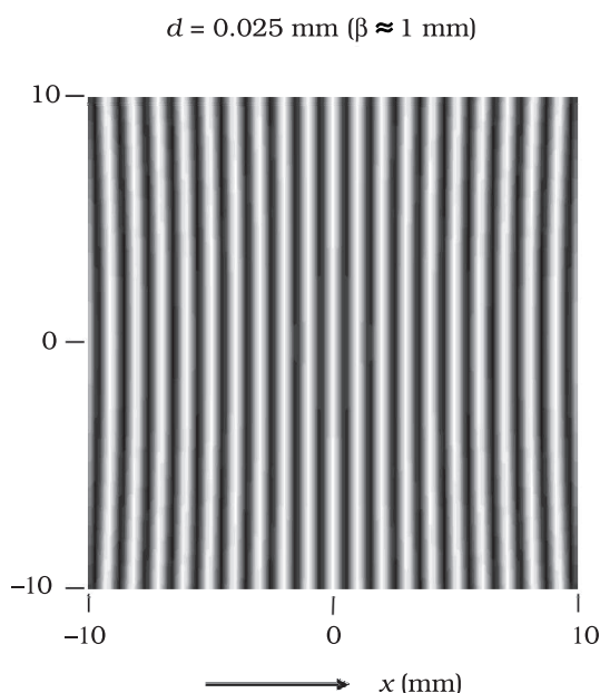
FIGURE 10.13 Computer generated fringe pattern produced by two point source S_1 and S_2 on the screen GG' (Fig. 10.12); d = 0.025 \text{ mm} , D = 5 \text{ cm} and \lambda = 5 \times 10^{-5} \text{ cm} .) (Adopted from OPTICS by A. Ghatak, Tata McGraw Hill Publishing Co. Ltd., New Delhi, 2000.)
