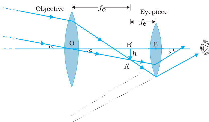
FIGURE 9.25 A refracting telescope.
