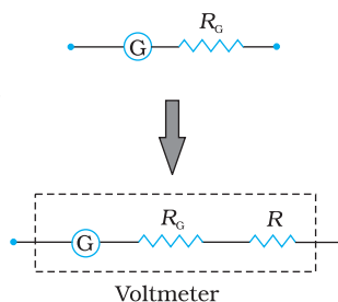
FIGURE 4.22 Conversion of a galvanometer (G) to a voltmeter by the introduction of a resistance R of large value in series.
